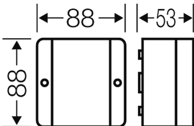
D9020 Dimension Drawing
